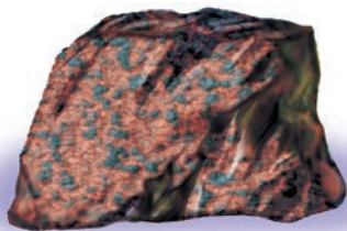
37-rasm. Granit.
