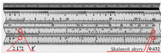
Logarifmik lineýka
